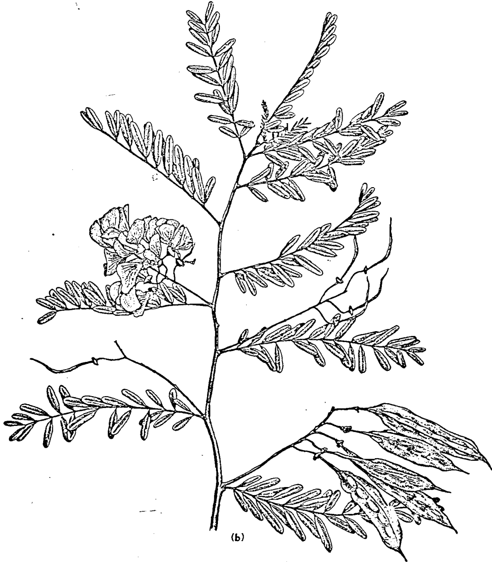
Fig. 100. Daubentonia punicea . (a) Distribution; (b) Habit sketch.
